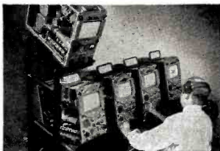
Compact GPL Cameras feature smooth operation, simplified control, (Swing-up and removable chassis permit easy servicing).
