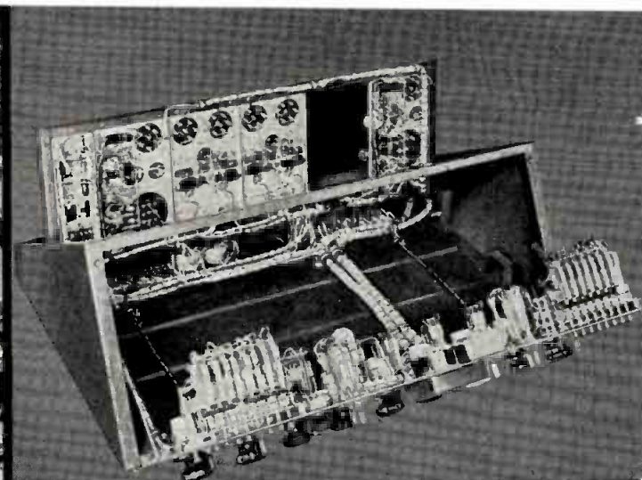
Accessibility, plus! New hinged control panel swings down; amplifier frame swings up.
